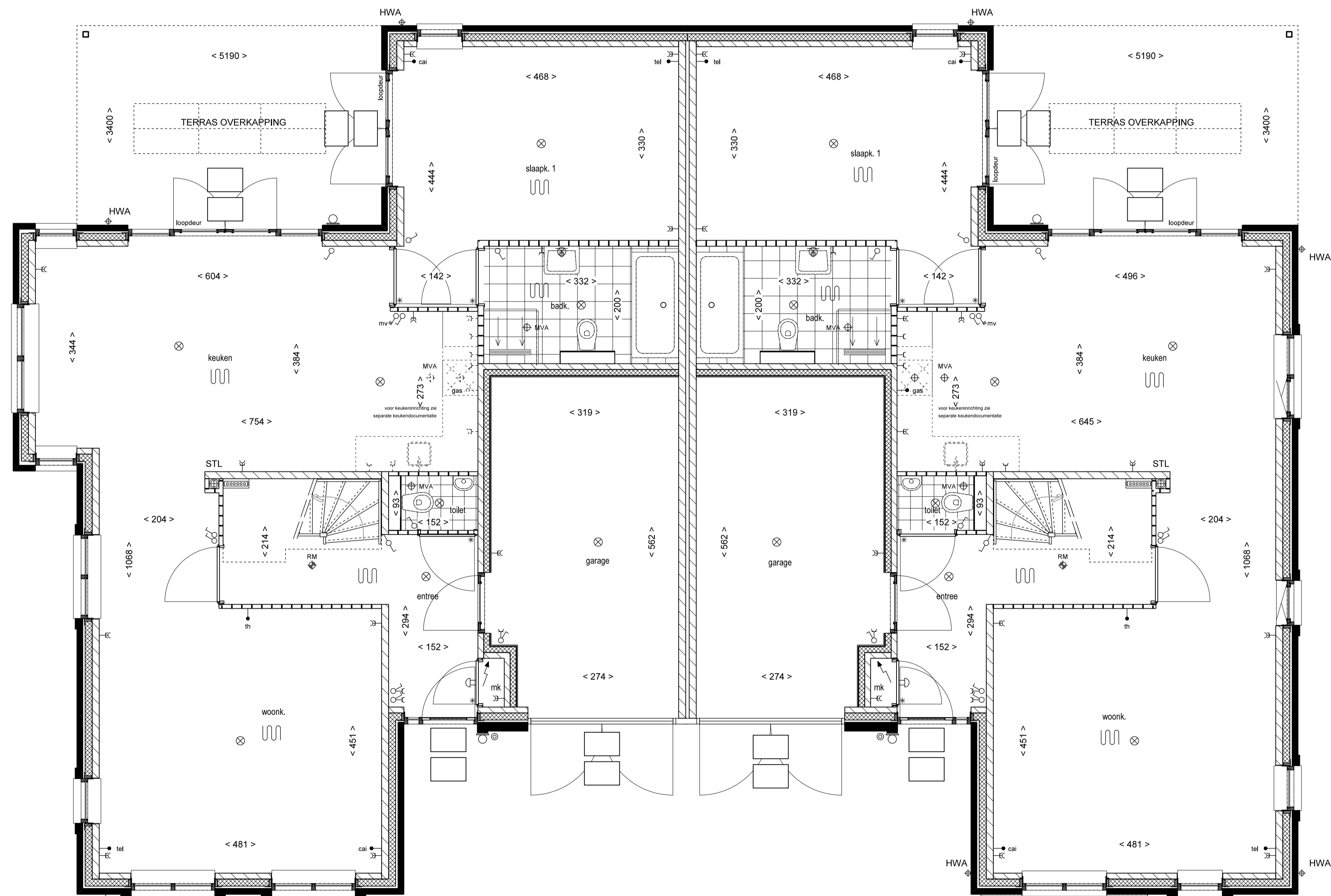
BEGANE GROND TYPE L2
